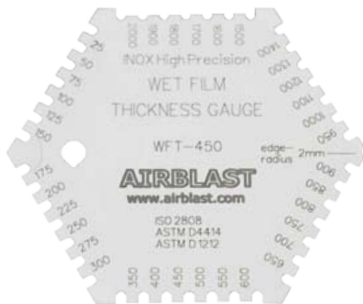
WFT-450
